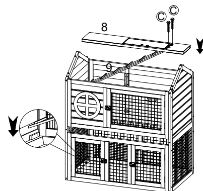
Step 3: Put down Mid-Floor & Ladder, Secure Ladder on Mid-Floor
