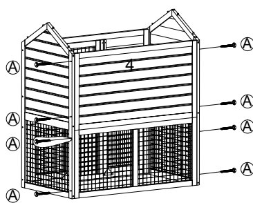
Step 2: Install the lower & Upper Back Panels
